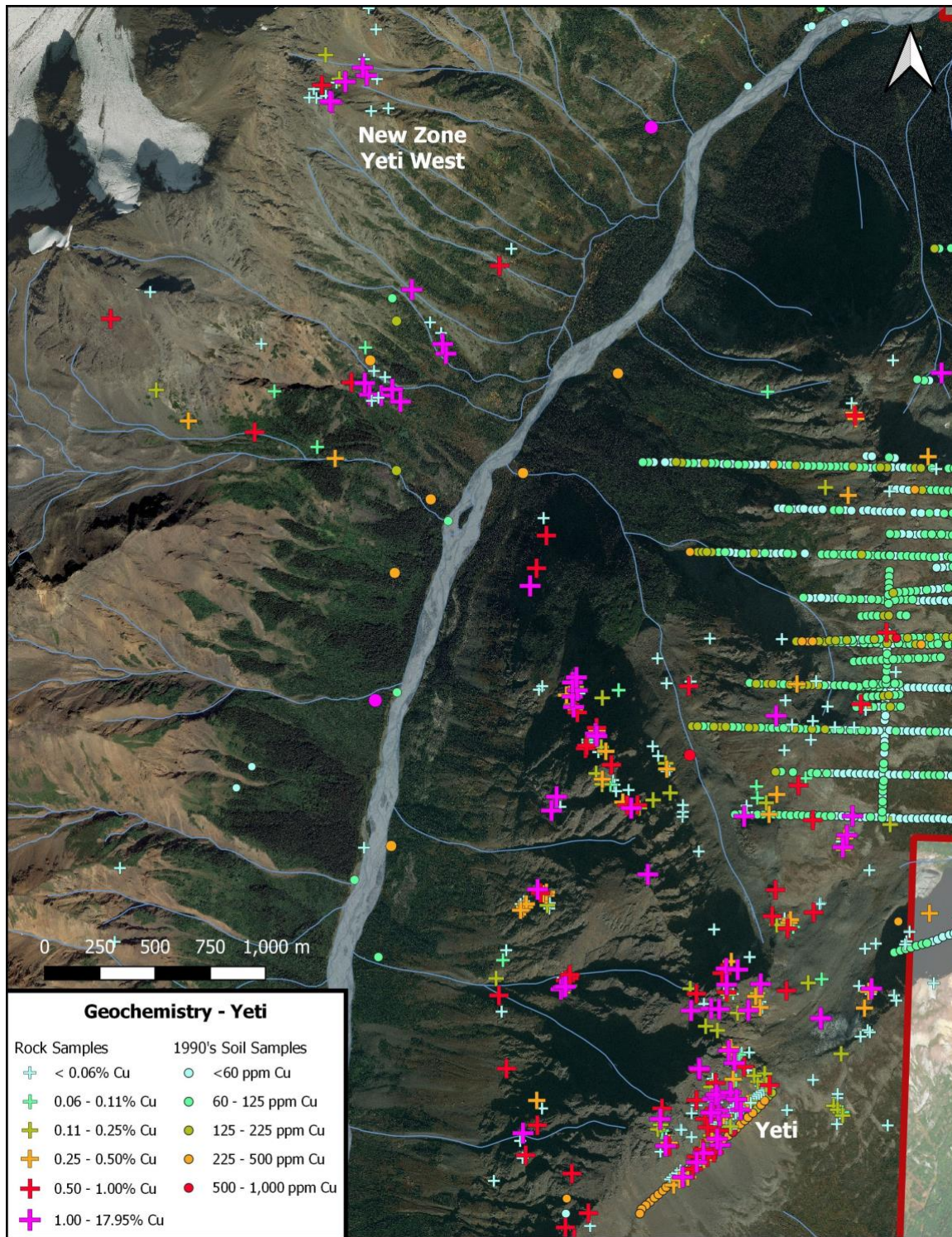
Figure 3 - Plan Map illustrating the Historic Soil and Historic and 2021 Rock Geochemistry of the Yeti Zone
