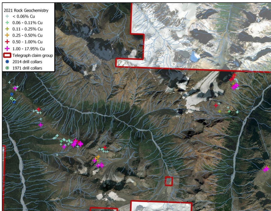
Figure 1 - Plan Map illustrating the 2021 Surface Rock Samples Locations and Copper Geochemistry Results
