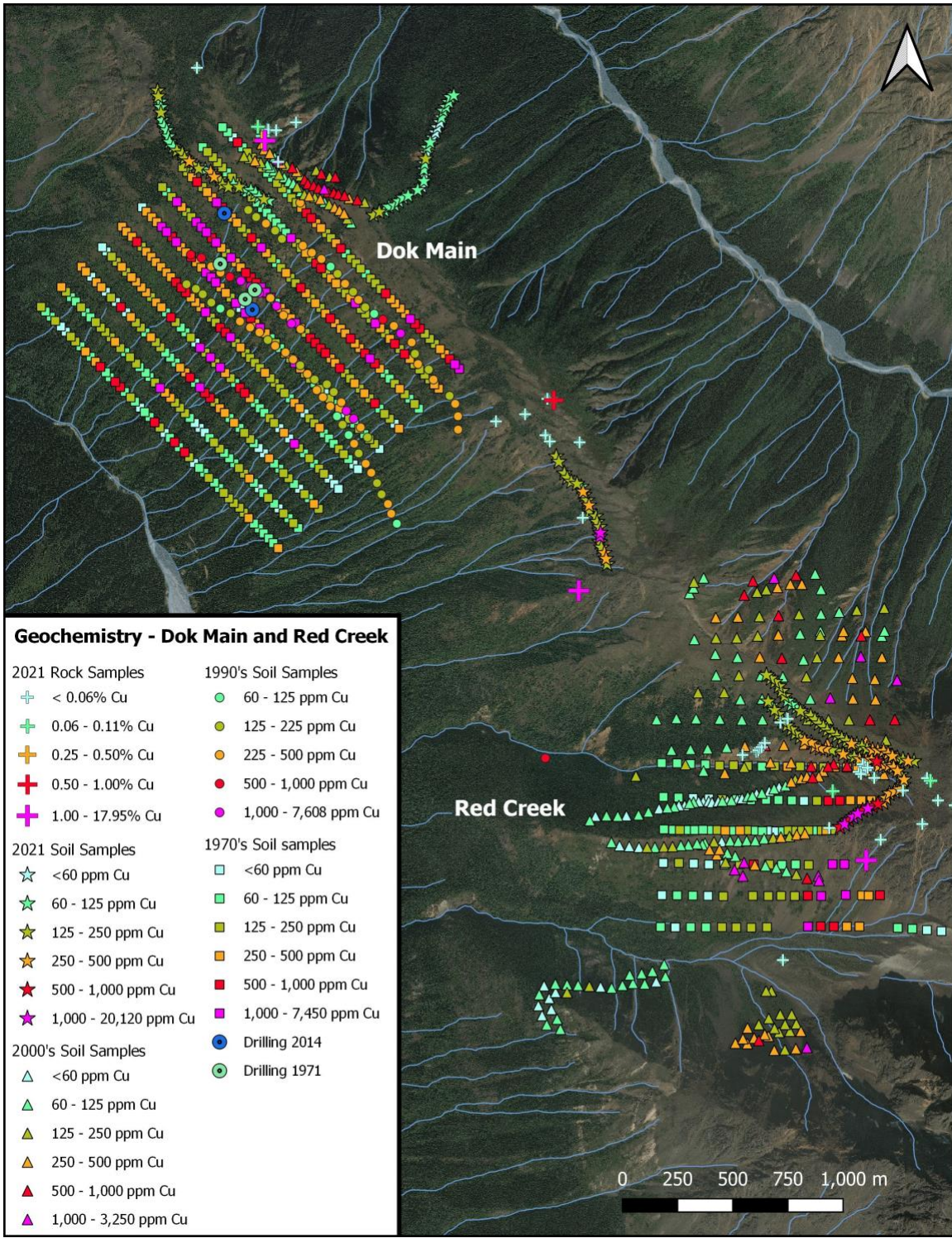
Figure 4 - Plan Map illustrating the Historic Soil and 2021 Rock Geochemistry of the DOK Main and Red Creek Zones
