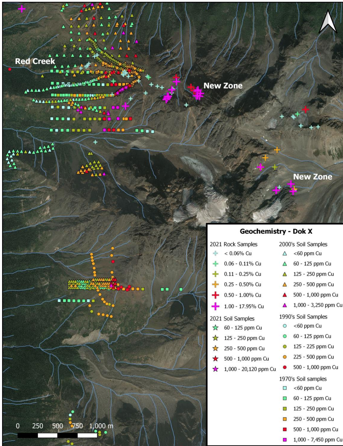
Figure 2 - Plan Map illustrating the Historic and 2021 Soil Geochemistry and the 2021 Rock Geochemistry of the DOK-X and 2021 Discovered Zones
